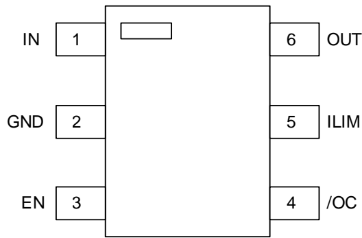
Figure 3. Pin Configuration (TOP VIEW)
