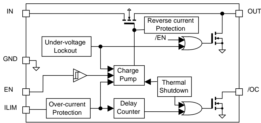
Figure 2. Block Diagram
