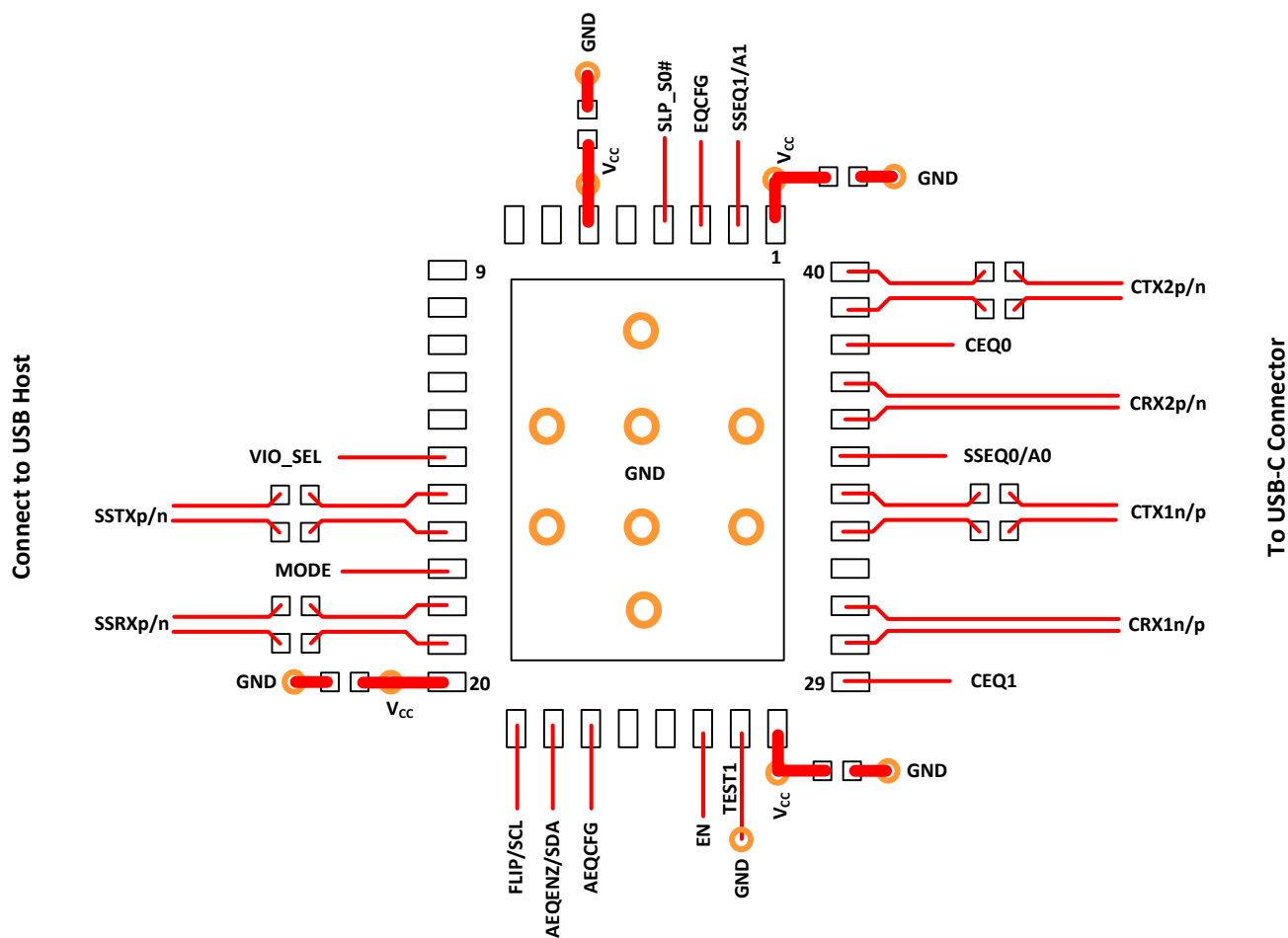
Figure 8-5. Layout Example
