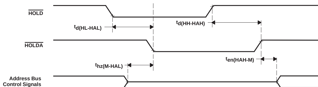
Figure 16. External DMA Timing for 'C203/'LC203
