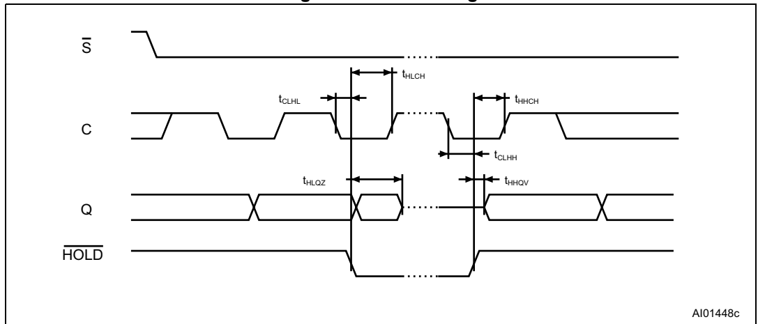
Figure 19. Hold timing
