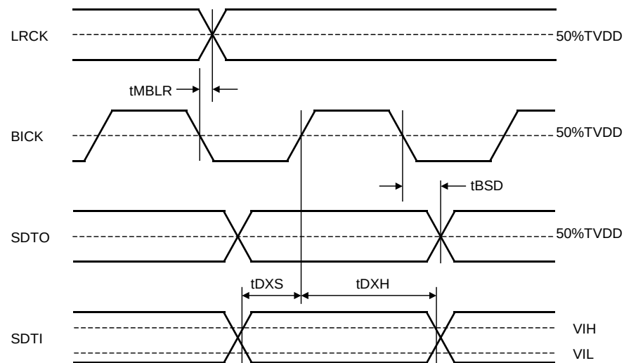
Audio Interface timing (Master Mode)
