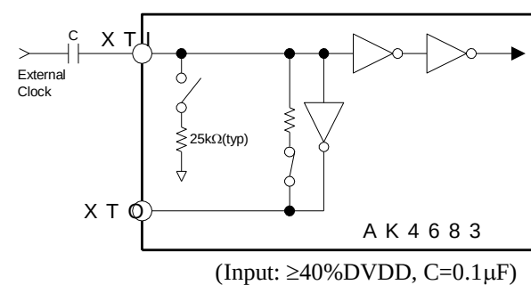
Figure 5. AC-coupled Input
