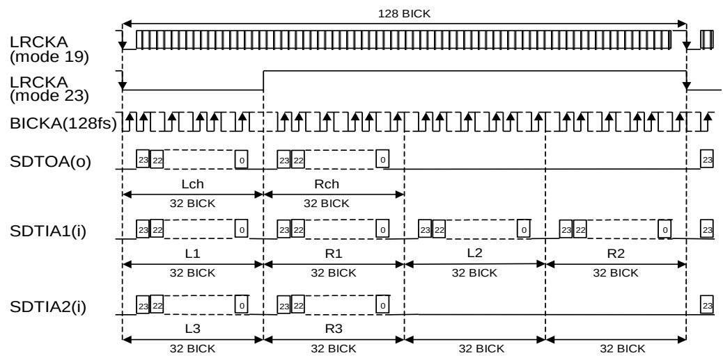
Figure 19. Mode 19 ,23 Timing
