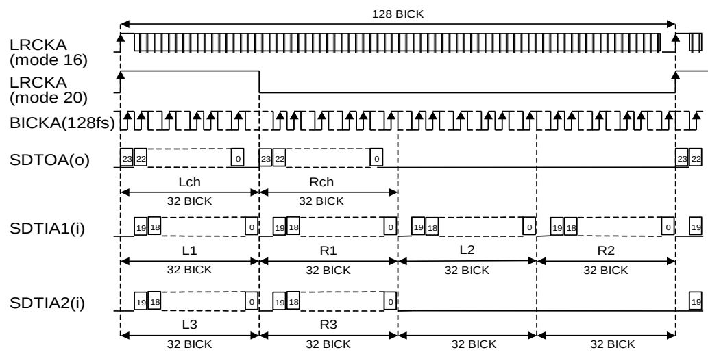
Figure 16. Mode 16 ,20 Timing
