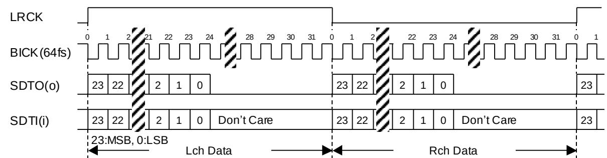
Figure 10. Mode 2,6 Timing
