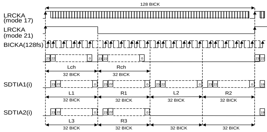
Figure 17. Mode 17 ,21 Timing
