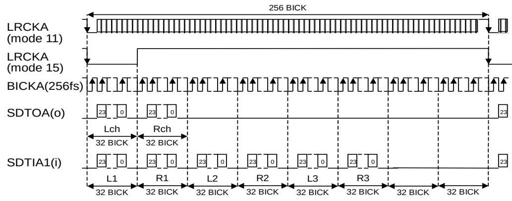
Figure 15. Mode 11 ,15 Timing
