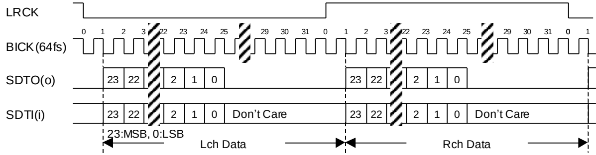
Figure 11. Mode 3 ,7 Timing
