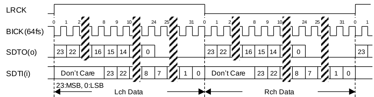
Figure 9. Mode 1,5 Timing
