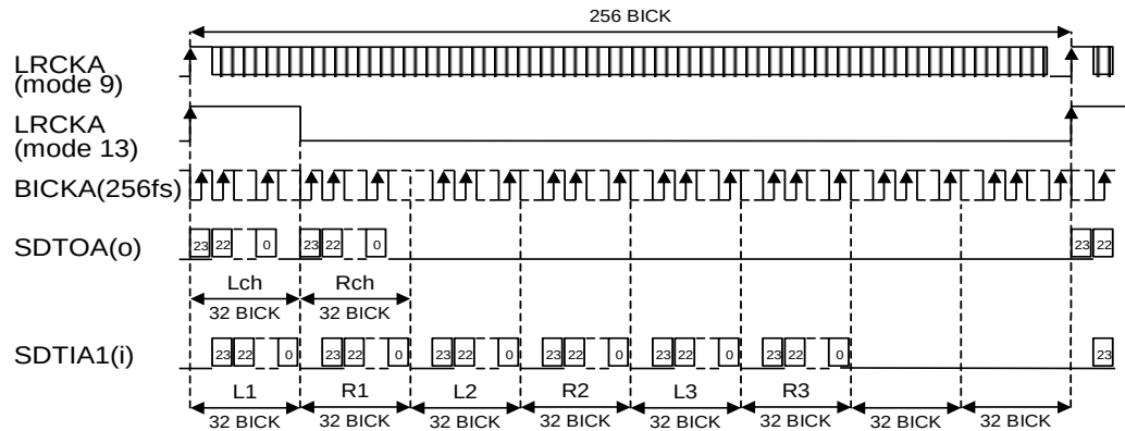
Figure 13. Mode 9 ,13 Timing
