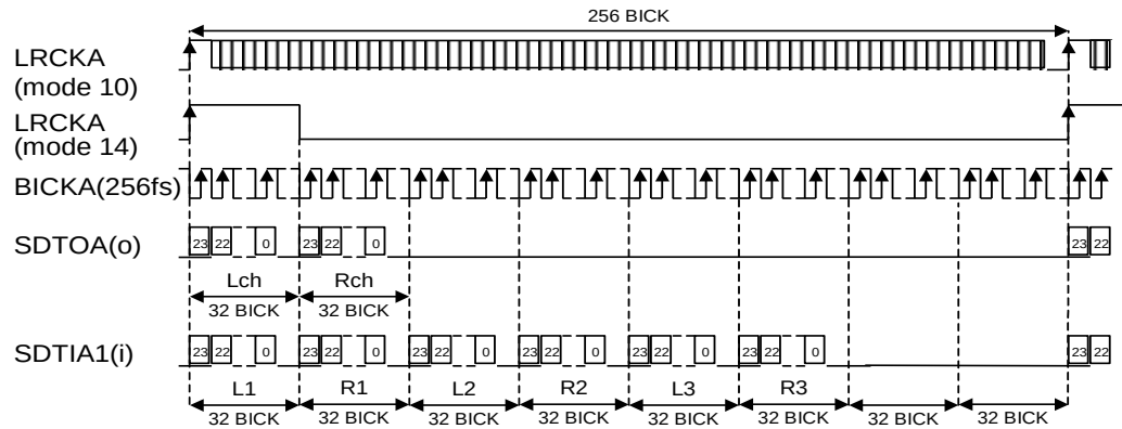
Figure 14. Mode 10 ,14 Timing
