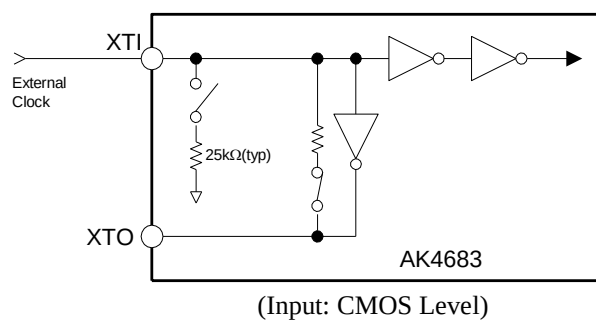
Figure 4. DC-coupled Input
