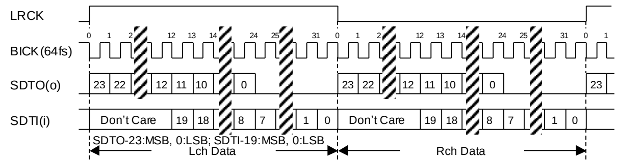
Figure 8. Mode 0,4 Timing
