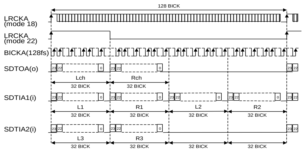
Figure 18. Mode 18 ,22 Timing
