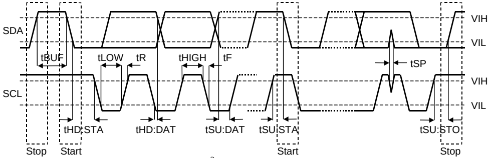
I 2 C Bus mode Timing The ADC/DAC part doesn't support READ command.
