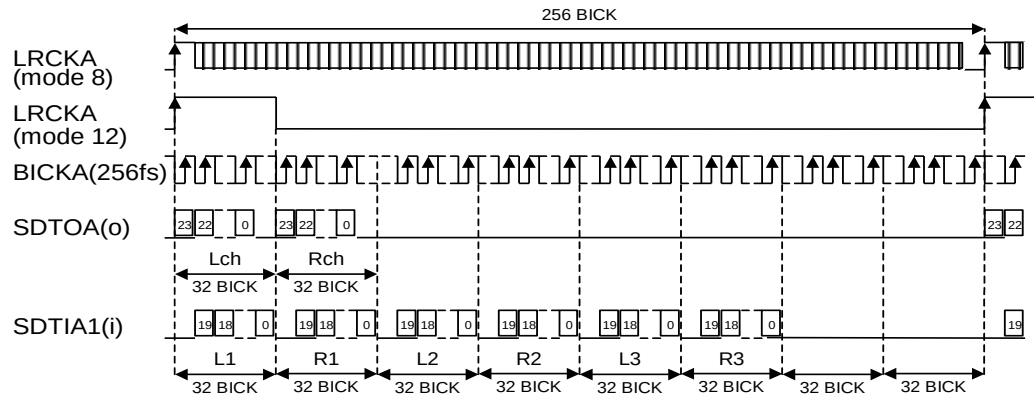
Figure 12. Mode 8 ,12 Timing
