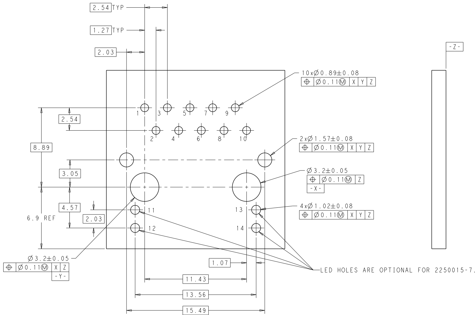
SUGGESTED CUSTOMER BOARD LAYOUT (COMPONENT SIDE)
