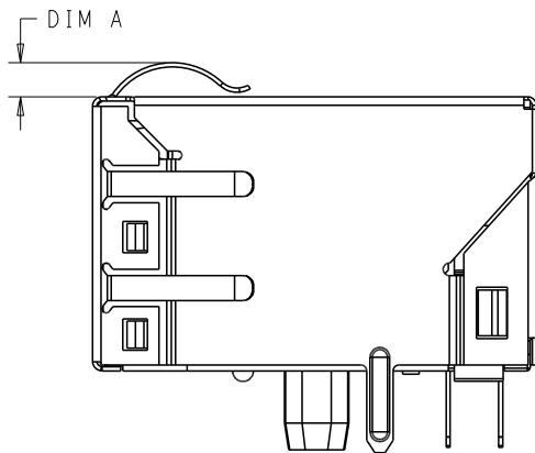
2250015-7 SHOWN (WITHOUT LED)
