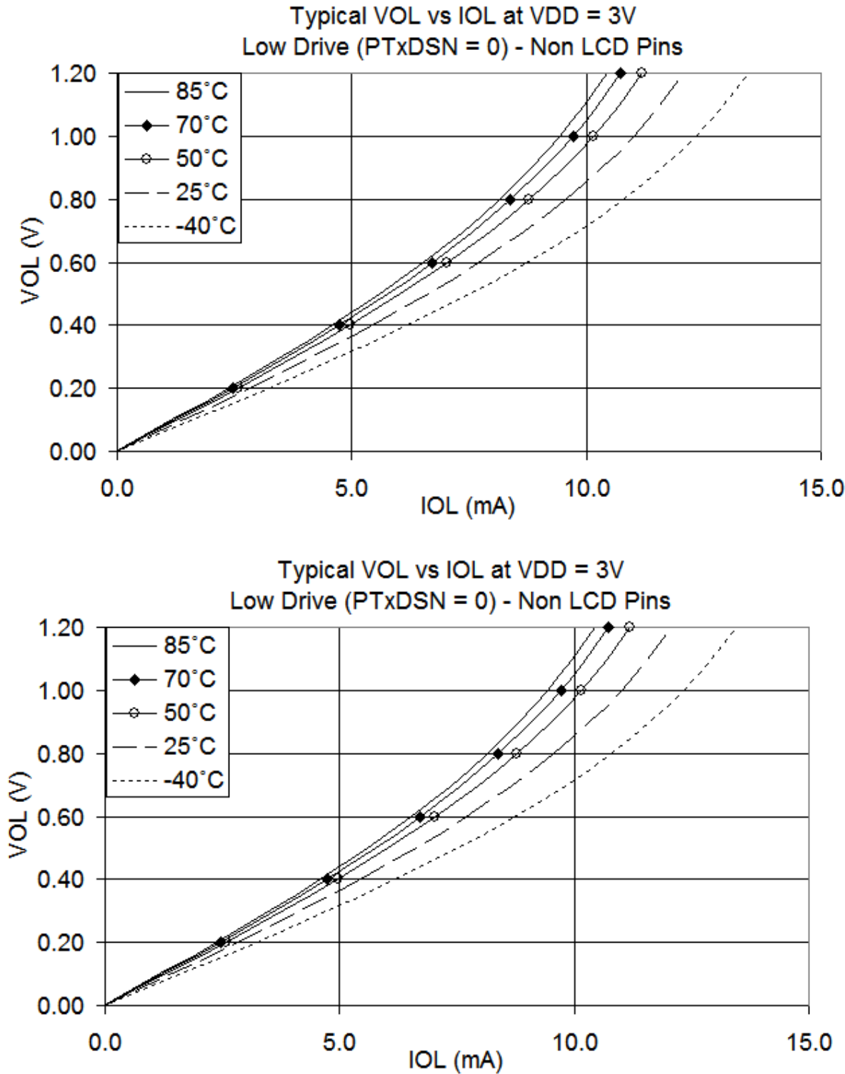
Figure 5. Typical Low-Side Driver (Sink) Characteristics (Non LCD Pins) — Low Drive (PTxDSn = 0)
