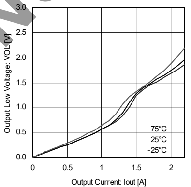
Fig.10 Output low voltage (BA6222)
