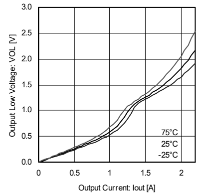
Fig.9 Output low voltage (BA6219BFP-Y)
