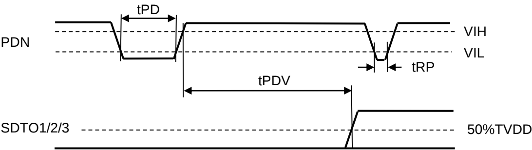
Figure 28. Power-down & Reset Timing
