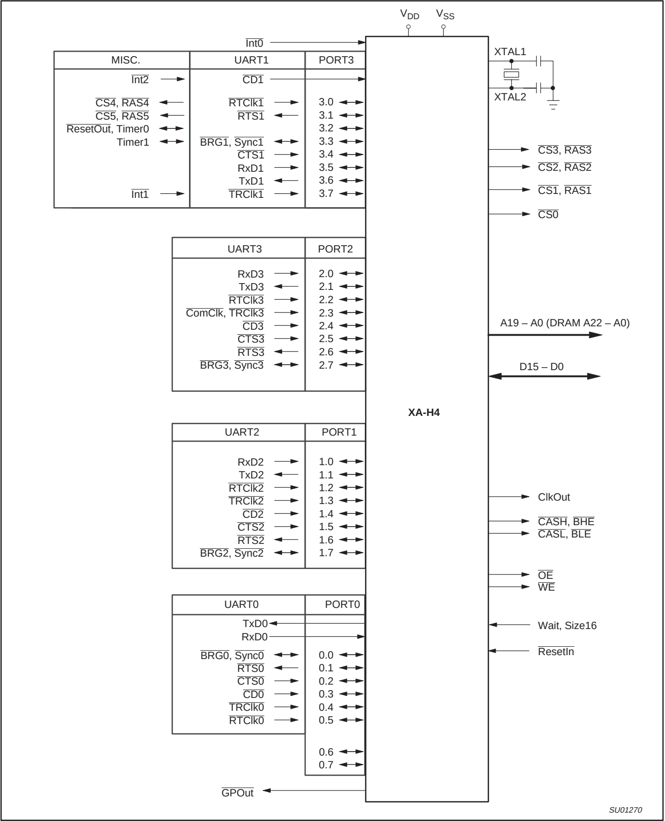
LOGIC SYMBOL XA-H4
