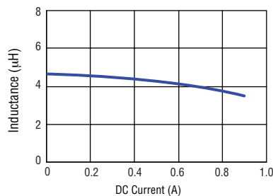
SRN2009T-4R7M
