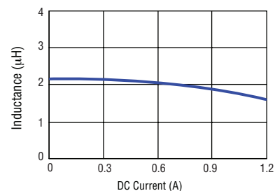
SRN2009T-2R2M
