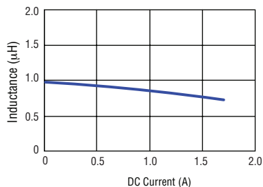
SRN2009T-1R0M
