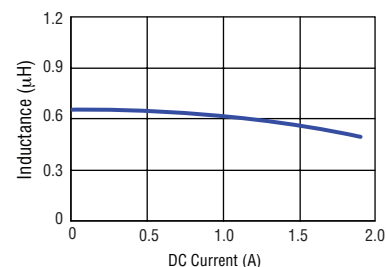
SRN2009T-R68M
