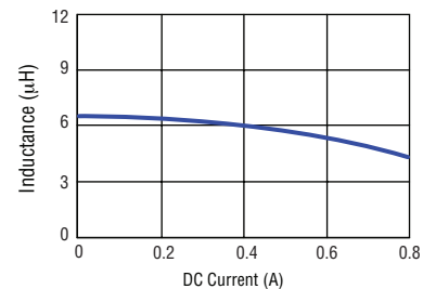
SRN2009T-6R8M
