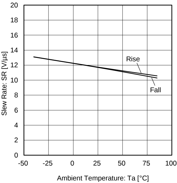
Figure 18. Slew Rate vs Ambient Temperature ( V_{DD} = 12\text{ V} )
