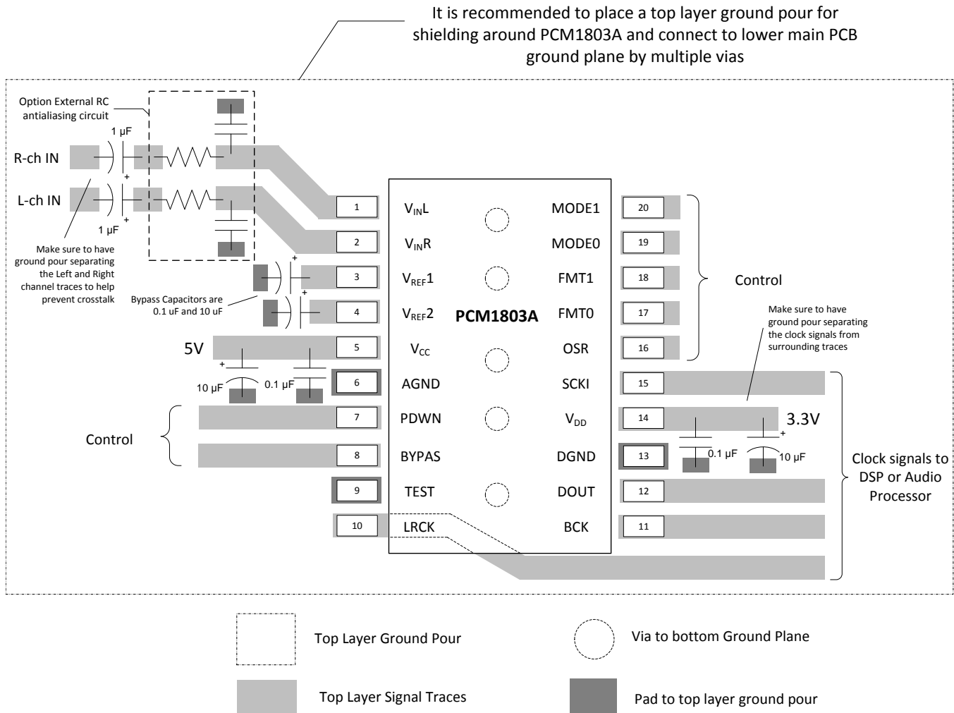
Figure 26. Layout Recommendation
