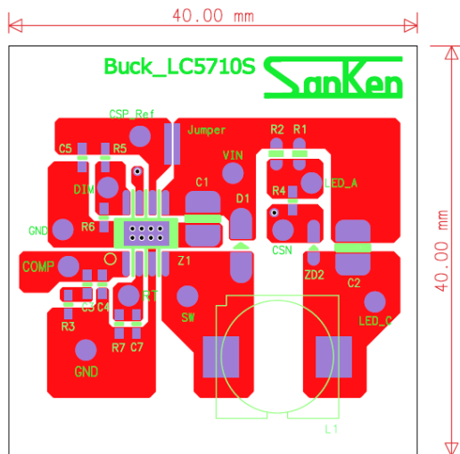
For Buck-type (parts mounting side)
