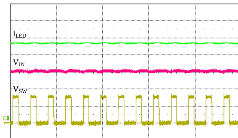
fig.28-21 Buck-mode
