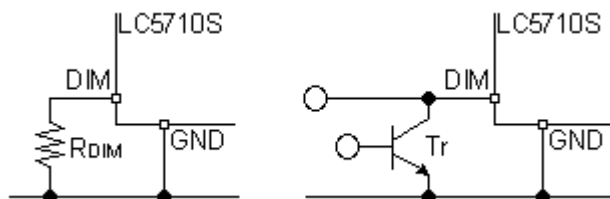
fig.8I The connection of R_{DIM} and remote ON/OFF application
