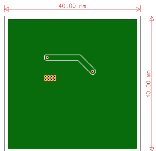
For Buck-type(back side)
