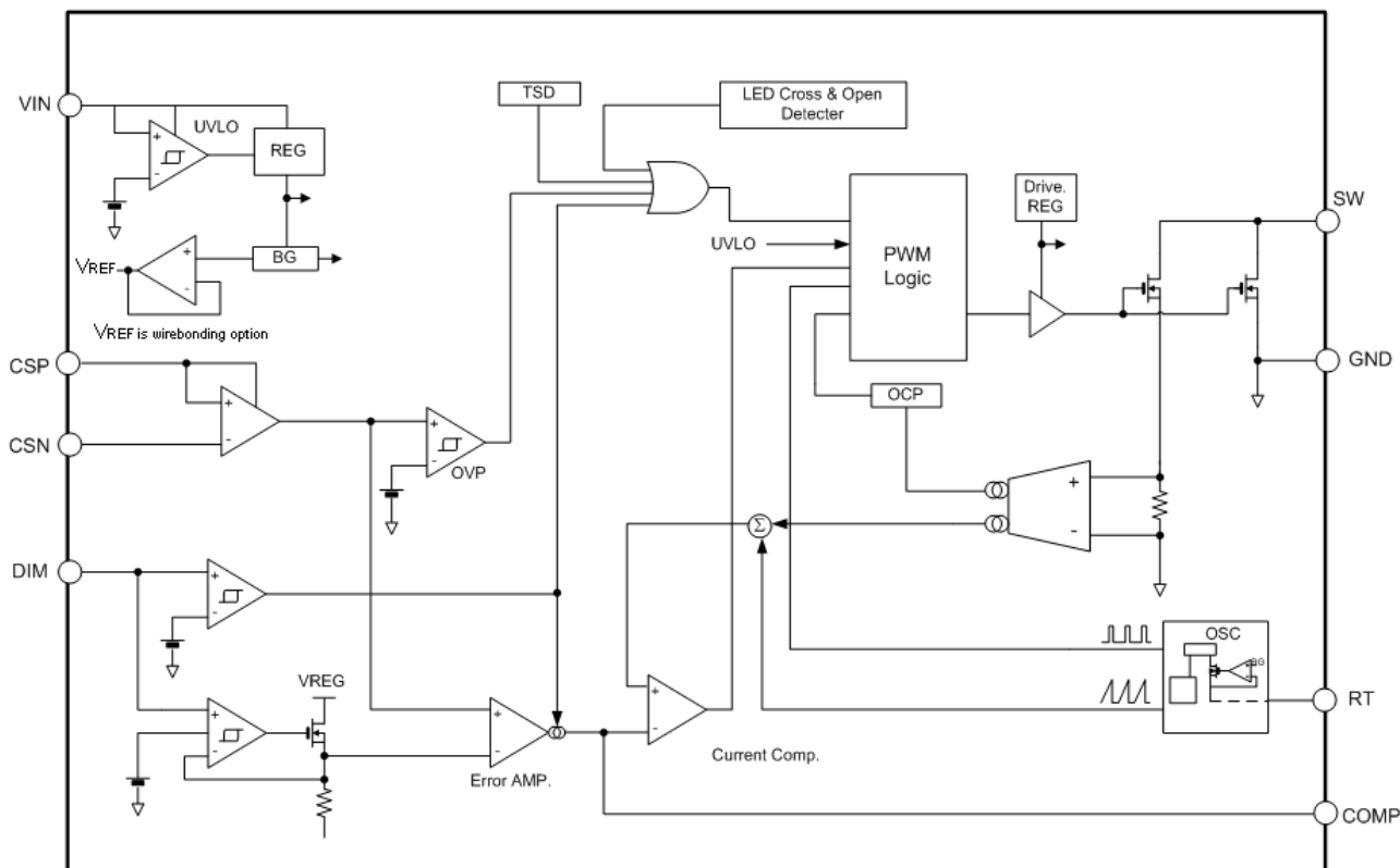
fig.2 Block diagram
