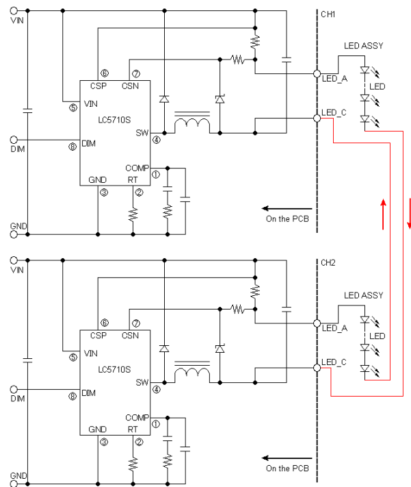
fig.20-2 Mis-wiring (Cross-connection)
