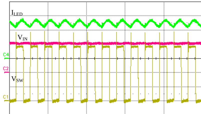
fig.28-25 Buck-boost-mode
