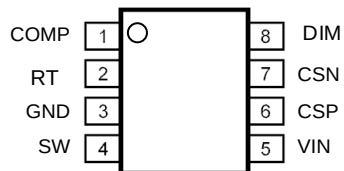
fig.3 Pin Assign
