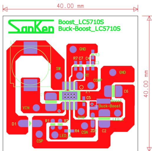
For Boost-type/Buckboost-type (parts mounting side)
