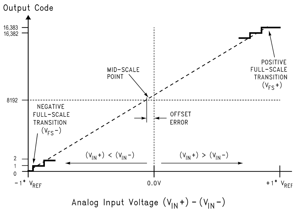
Figure 2. Transfer Characteristic (Offset Binary Format)
