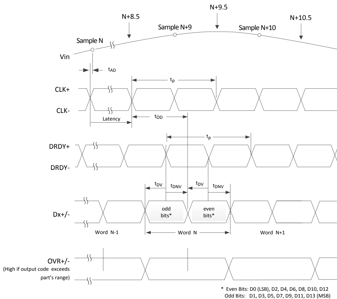
Figure 1. Output Timing
