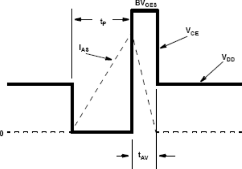
Figure 20. Energy Waveforms
