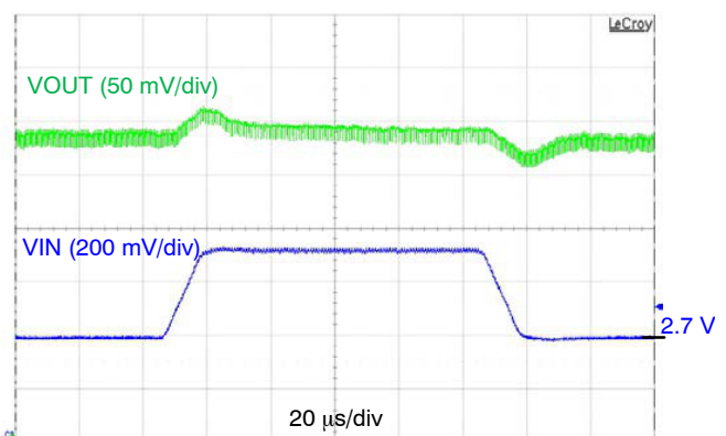
Figure 38. Line Transient, 2.7–3.0 V_{IN} , 10 \mu\text{s} Edge, 500 mA Load, V_{OUT} = 3.3\text{ V}
