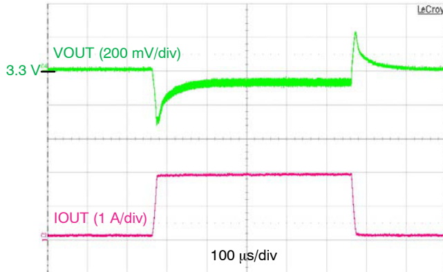
Figure 35. Load Transient, 150–2000 mA, 10 \mu\text{s} Edge, V_{IN} = 3.0\text{ V} , V_{OUT} = 3.3\text{ V}
