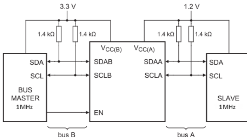
Figure 9: Typical Application
