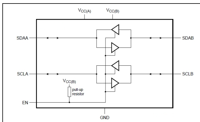
Figure 1: Block Diagram
