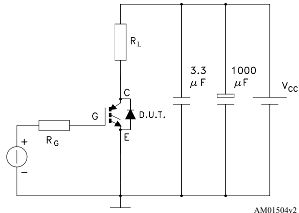
Figure 15. Test circuit for resistive load switching
