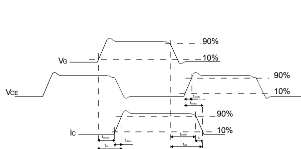
Figure 17. Switching waveform
