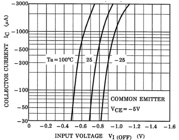
Fig. 10.4 RN2907FE I_C - V_{I(OFF)}
