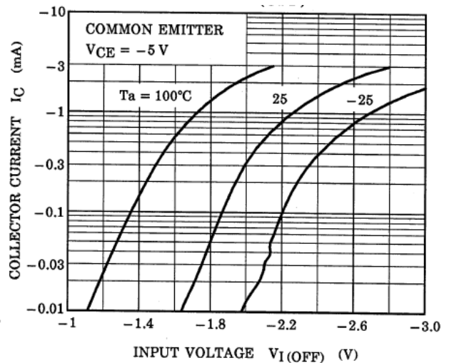
Fig. 10.6 RN2909FE I_C - V_{I(OFF)}
