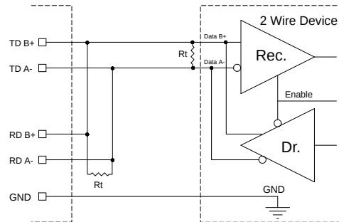
Figure 1: Typical RS-485 Two-Wire Setup
