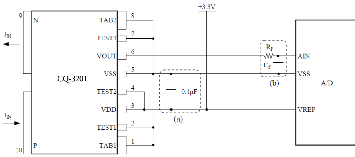
Figure 8. Recommended external circuits of CQ-3201.
