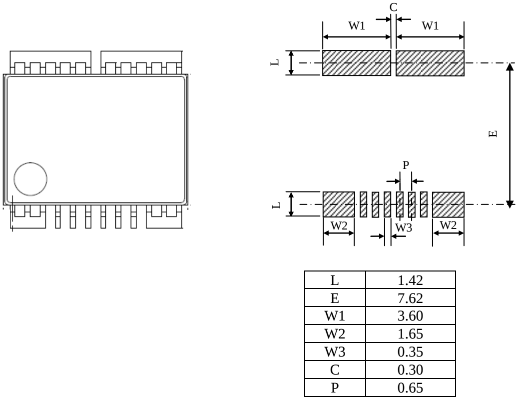
Figure 10. Pad dimensions of CQ-3201.
