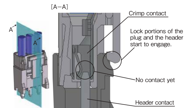
Lock structure
