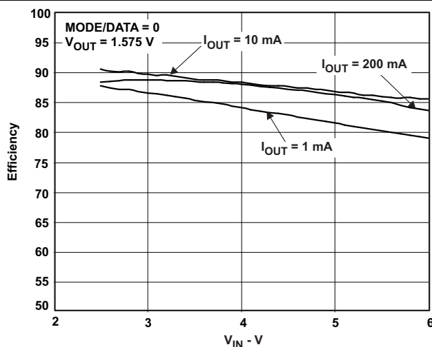
Figure 19. Efficiency vs V_{IN} , V_{OUT1} = 1.575\text{ V}
