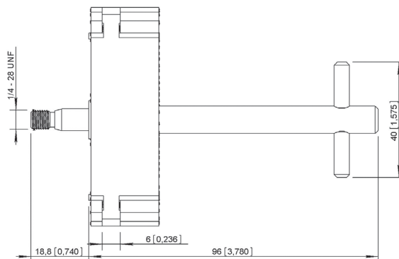
Central jackscrew
