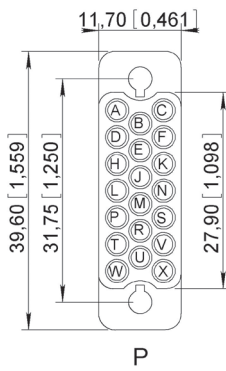
20 contacts
