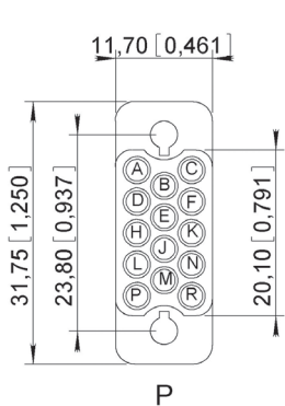
14 contacts
