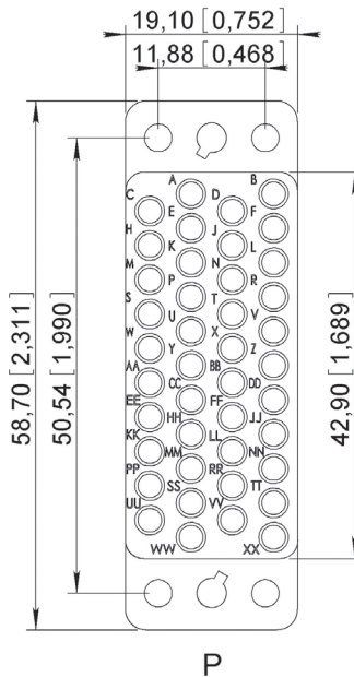
42 contacts
