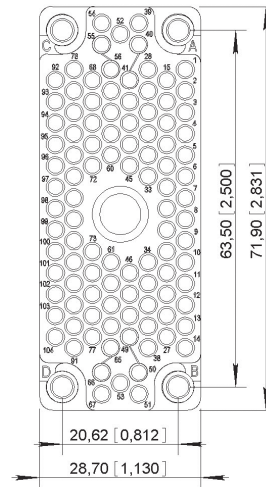
Central jackscrew
