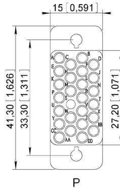
26 contacts
