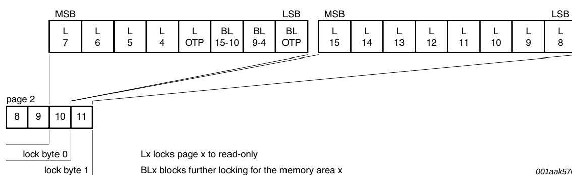
Fig 7. Lock bytes
