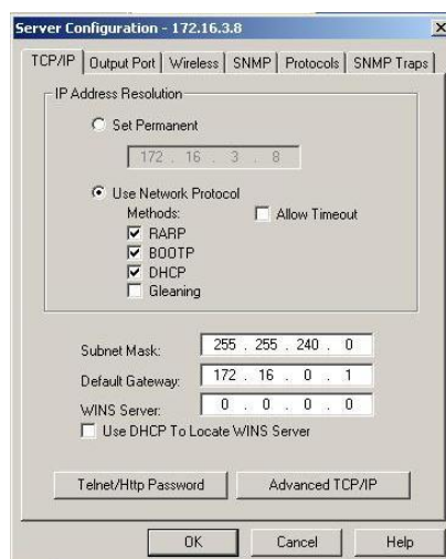
Figure 14 TCP/IP Window
