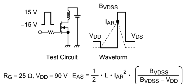
Fig. 8.16 Test Circuit/Waveform
