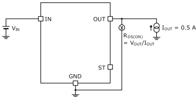
Measurement Circuit for Figure 6, Figure 7
