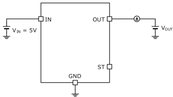
Measurement Circuit for Figure 18, Figure 19
