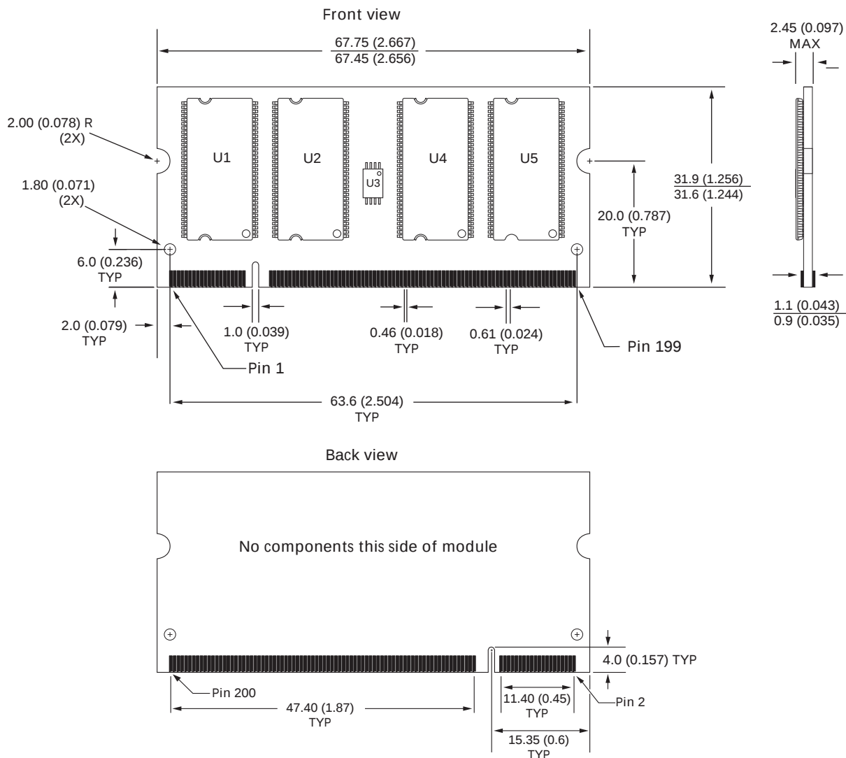
Figure 3: 200-Pin SODIMM
