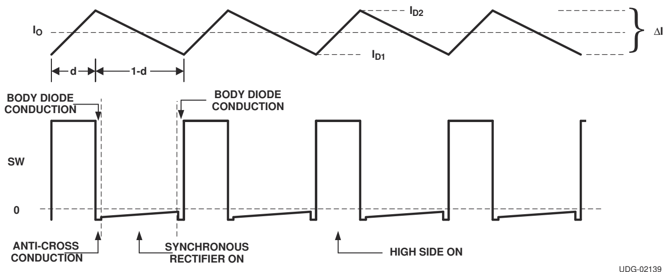
Figure 8-1. Inductor Current and SW Node Waveforms
