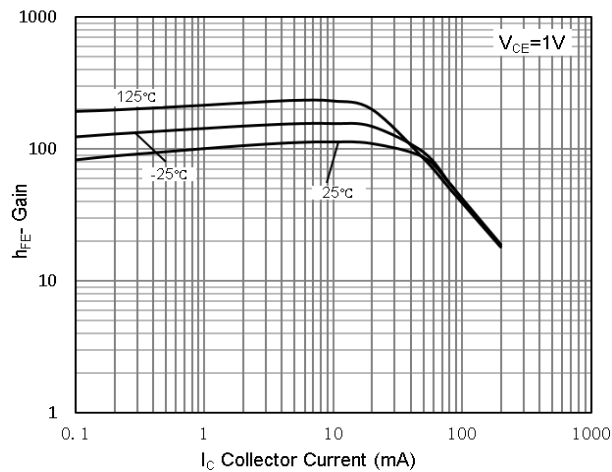
Fig.5 h_{FE} vs I_C
