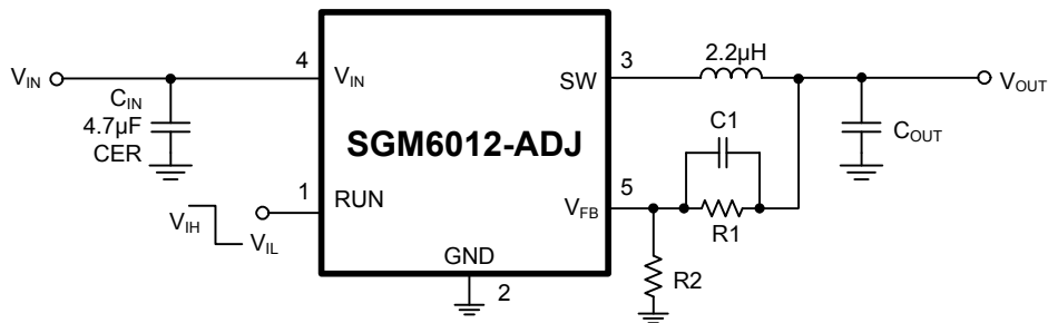
Figure 4. Basic Application Circuit with Adjustable Version
