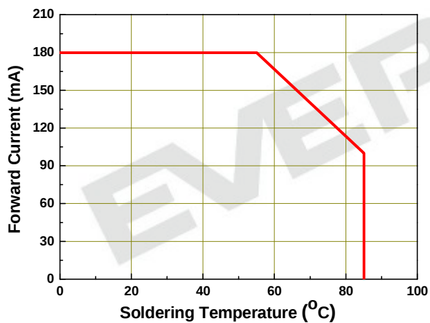
Fig.5 – Max. Driving Forward Current vs. Soldering Temperature
