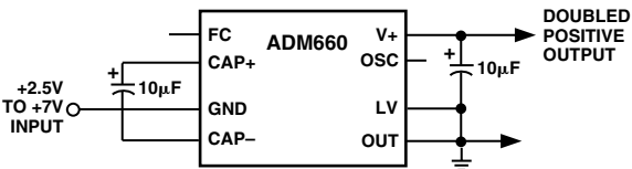
Figure 8. Voltage Doubler Configuration
