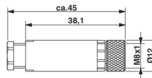
Dimensional drawing
