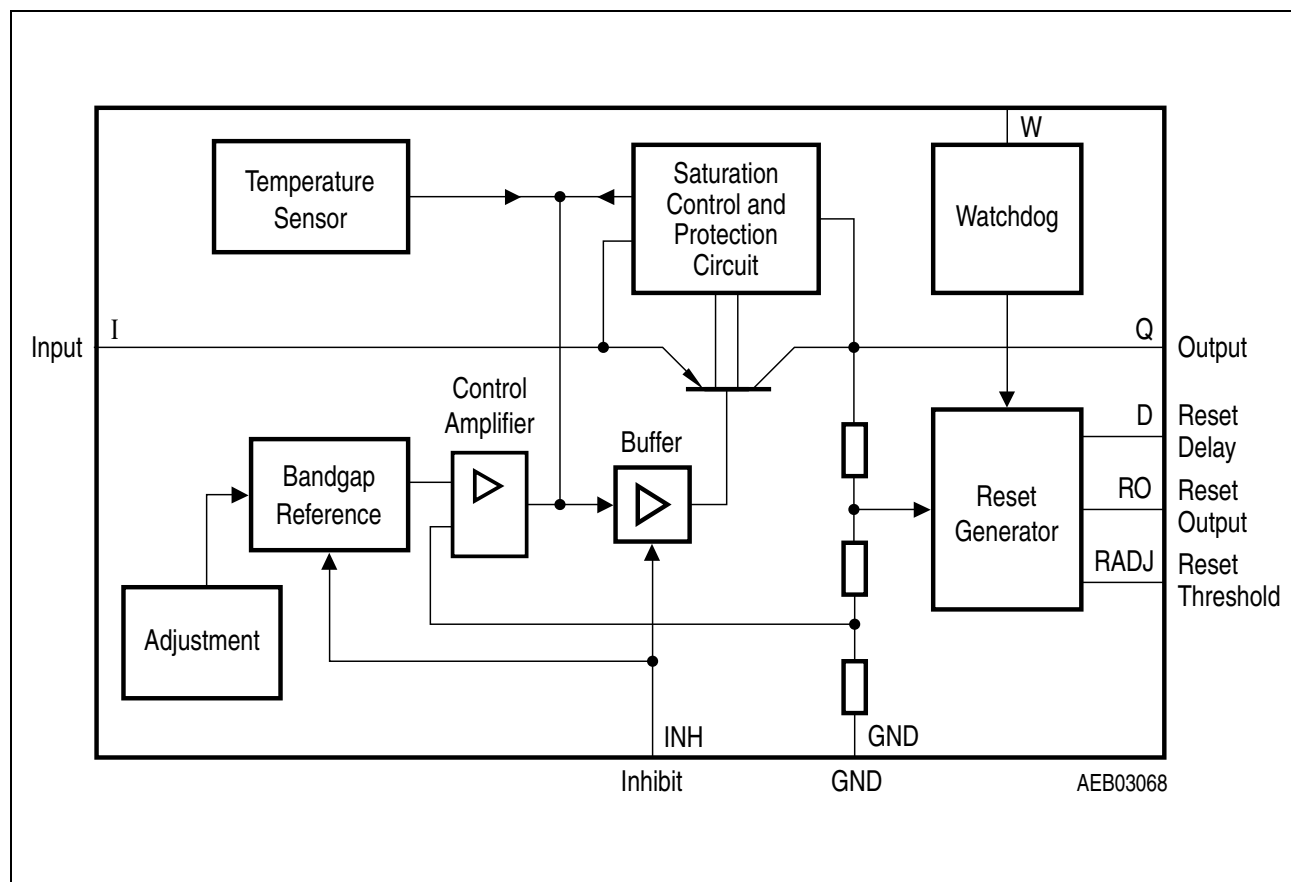
Figure 2 Block Diagram
