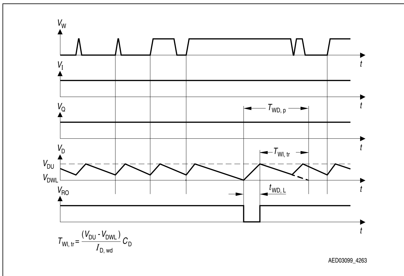
Figure 6 Timing of the Watchdog Function Reset
