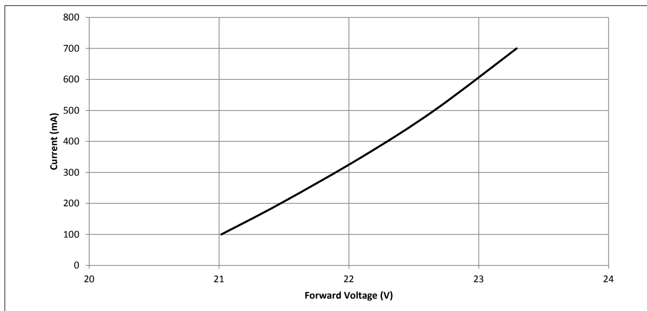
Figure 1: Drive Current vs. Voltage ( T_{c2} = 50^{\circ}\text{C} ) for Lo280 modules
