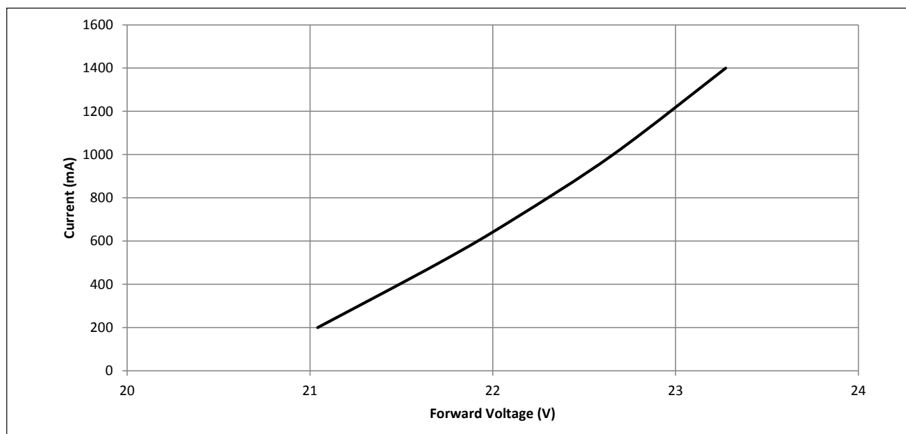
Figure 2: Drive Current vs. Voltage ( T_{c2} = 50^{\circ}\text{C} ) for Lo560 modules
