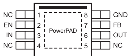
Pin Functions
