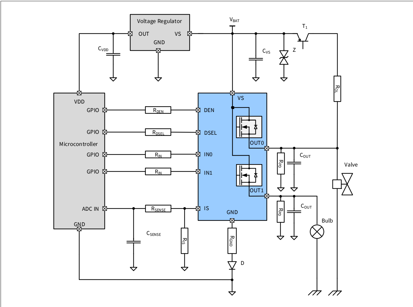
Figure 53 Application Diagram with BTT6030-2ERB
