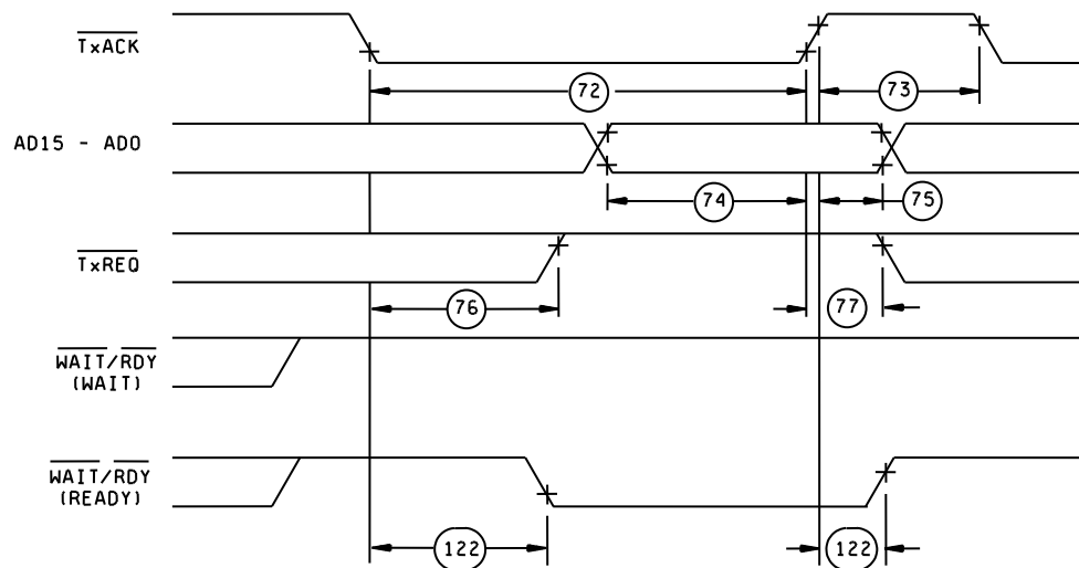
DMA WRITE CYCLE
