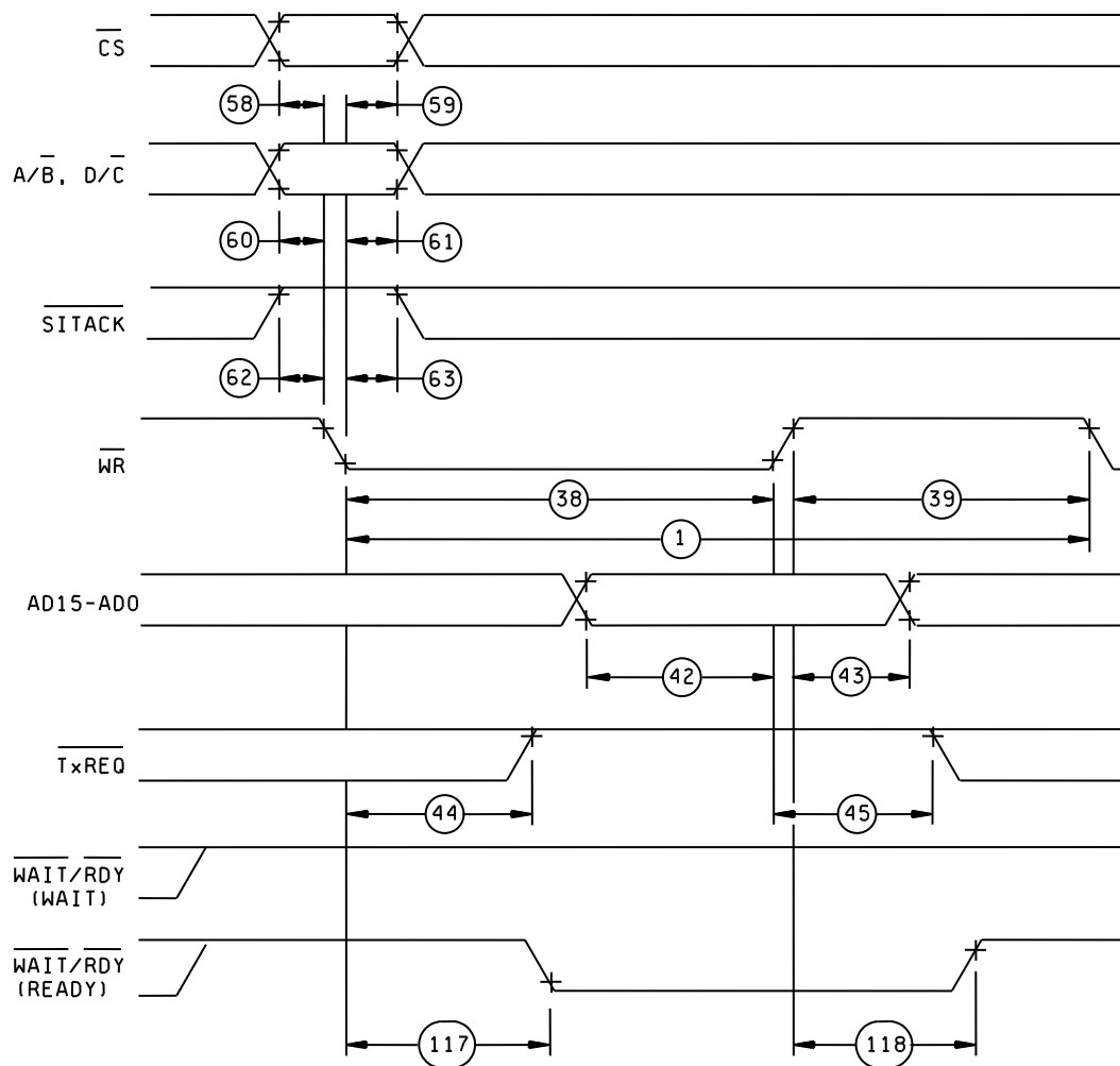
NON-MULTIPLEXED \overline{\text{WR}} WRITE CYCLE
