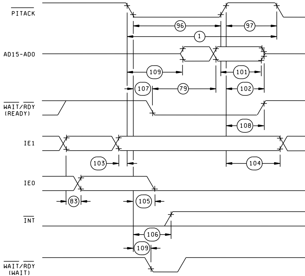
NON-MUX RD INTERRUPT ACKNOWLEDGE CYCLE
