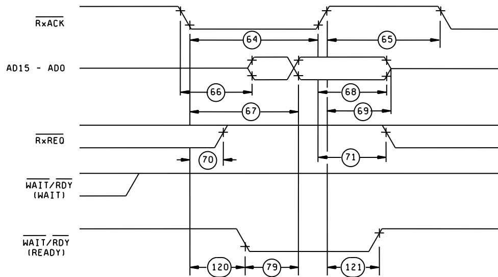
DMA READ CYCLE
