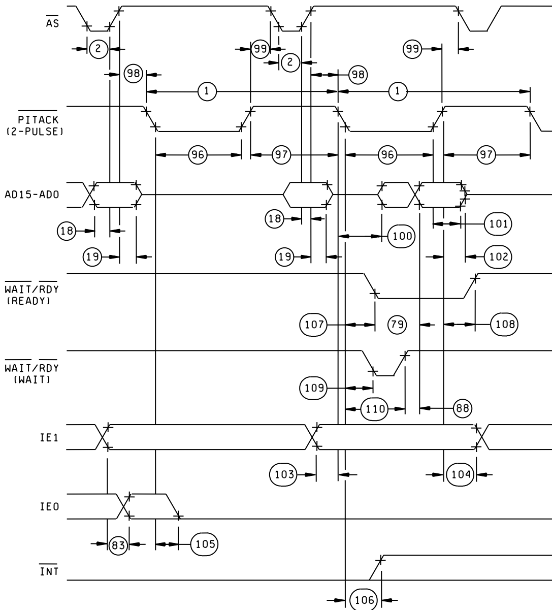
MULTIPLEXED DOUBLE-PULSE INTACK CYCLE
