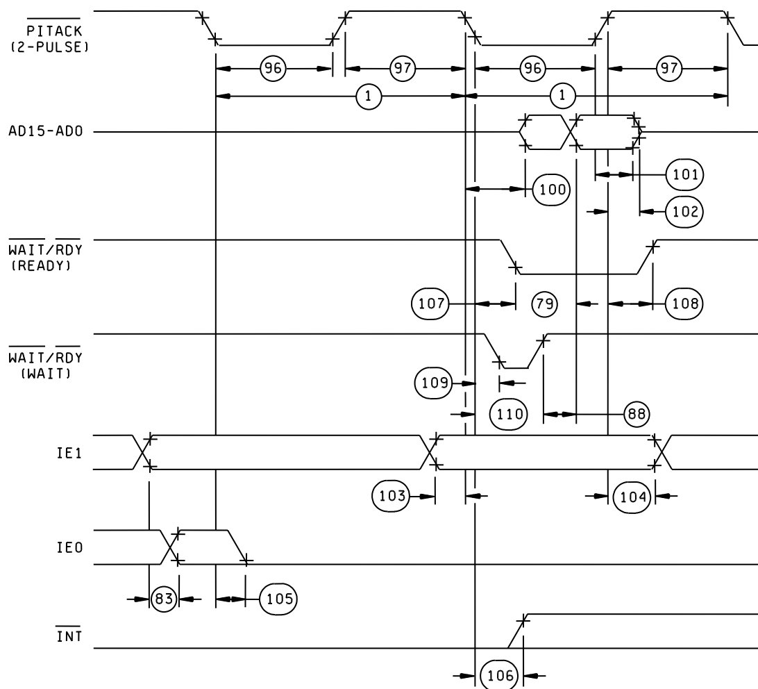
NON-MULTILPEXED DOUBLE-PULSE INTACK CYCLE
