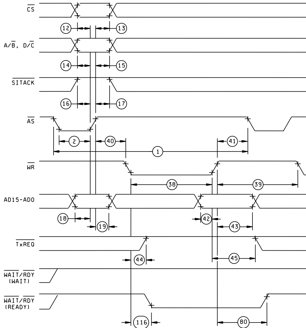
MULTIPLEXED \overline{\text{WR}} WRITE CYCLE
