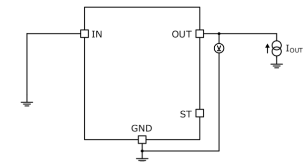
Measurement Circuit for Figure 8, Figure 9
