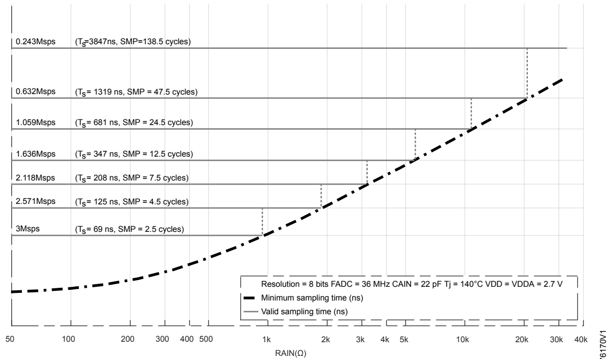
Figure 25. Minimum sampling time versus RAIN for 8 bits resolution
