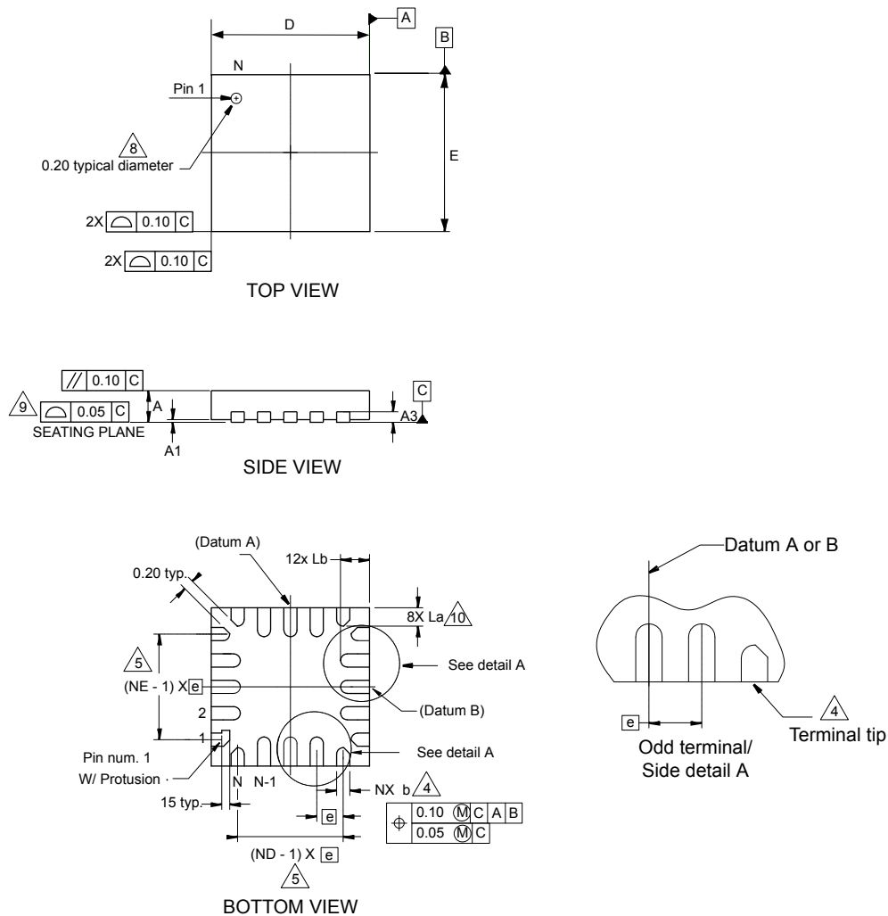
Figure 39. UFQFPN20 - Outline
