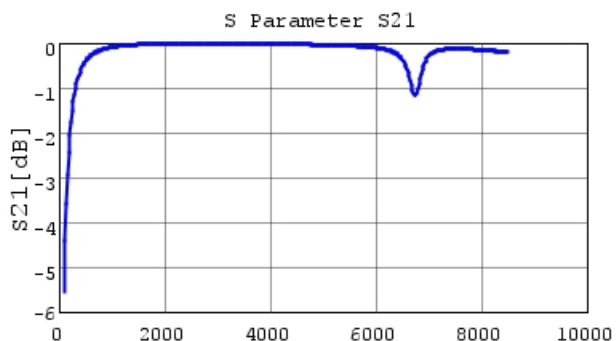
GCQ1555C1H9R9DB01 S21 DCOV, 25degC
