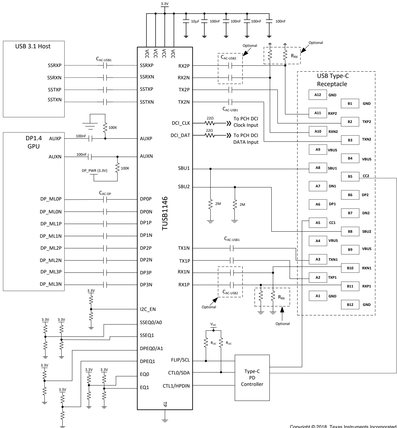
Figure 34. Application Circuit
