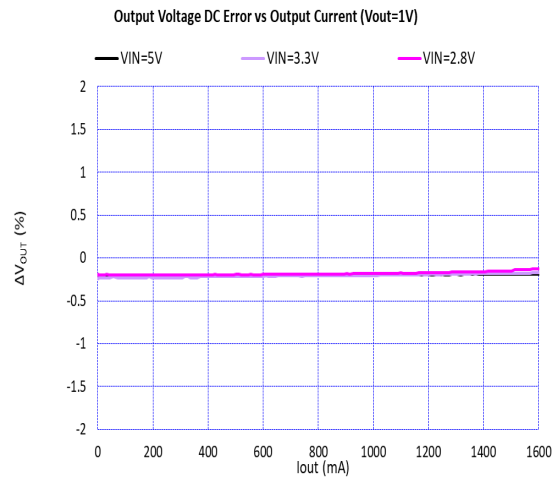
Figure 30. Output Voltage DC Error vs Output Current ( V_{OUT} = 1.0 V , T_A = 25^{\circ}C )
