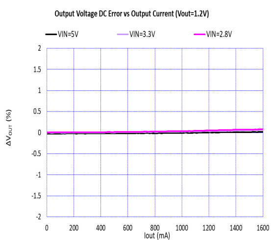
Figure 32. Output Voltage DC Error vs Output Current ( V_{OUT} = 1.2 V , T_A = 25^{\circ}C )
