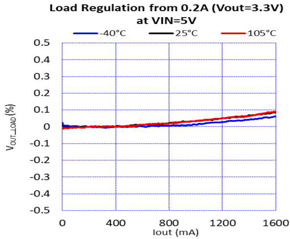
Figure 29. Load Regulation ( V_{IN} = 5.0 V , V_{OUT} = 3.3 V )
