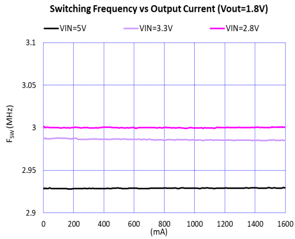
Figure 35. Switching Frequency vs Output Current ( V_{OUT} = 1.8\text{ V} , T_A = 25^\circ\text{C} )
