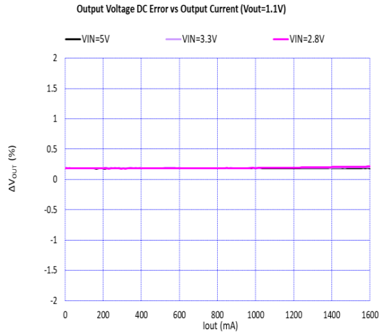
Figure 31. Output Voltage DC Error vs Output Current ( V_{OUT} = 1.1 V , T_A = 25^{\circ}C )
