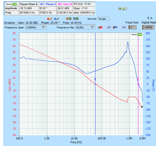
Figure 69. Bode Plot NCV6323FxmLMTW18TBG L = 1.0 \mu H – COUT = 100 \mu F
