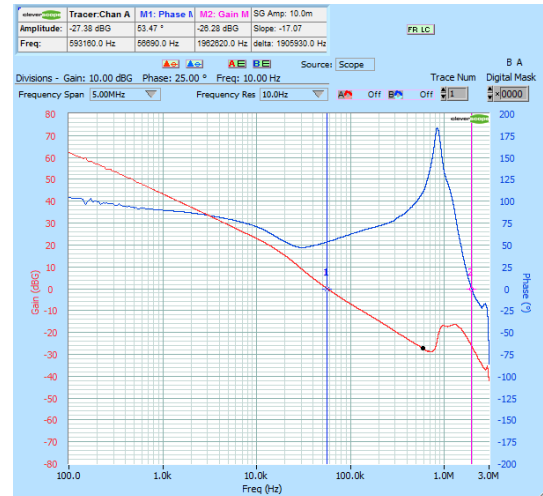
Figure 75. Bode Plot NCV6323FxmLMTW10TBG L = 1.0 \mu H – COUT = 100 \mu F
