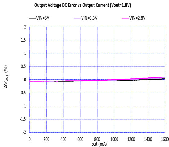
Figure 33. Output Voltage DC Error vs Output Current ( V_{OUT} = 1.8 V , T_A = 25^{\circ}C )
