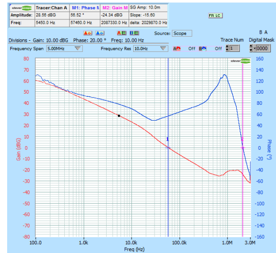
Figure 73. Bode Plot NCV6323FxmLMTW12TBG L = 1.0 \mu H – COUT = 100 \mu F
