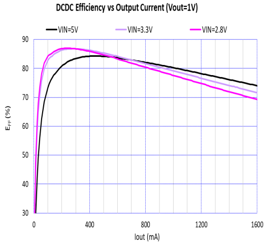
Figure 11. Efficiency vs. Output Current and Input Voltage ( V_{OUT} = 1.0\text{ V} , T_A = 25^\circ\text{C} , L = \text{FDSD0420-H-1R0M} )
