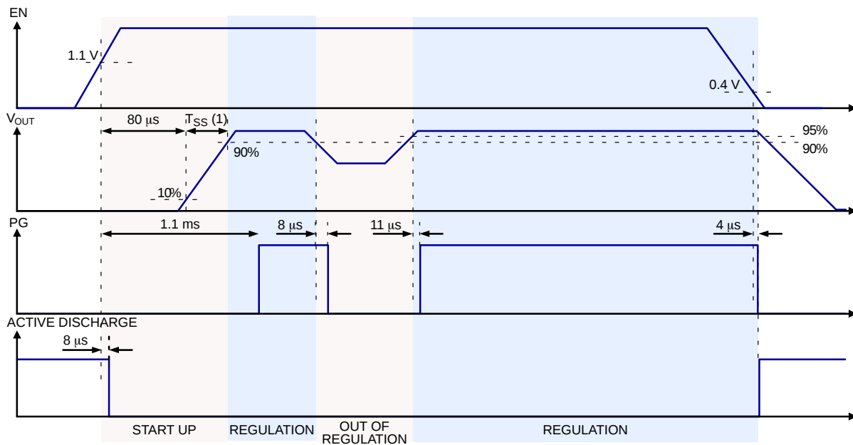
Figure 78. Power Good and Active Discharge Timing Diagrams
