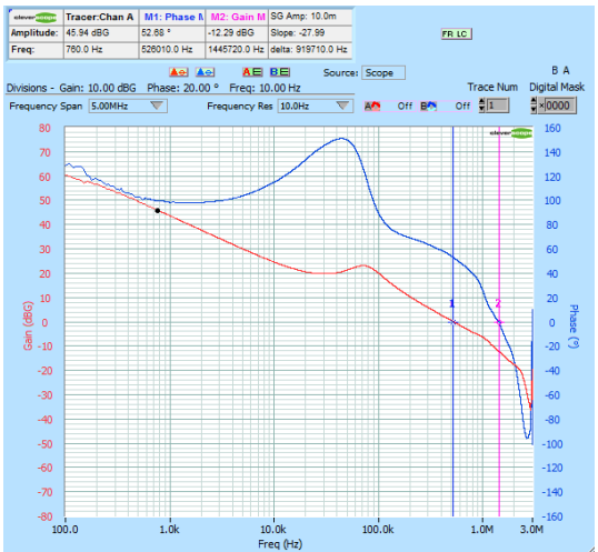
Figure 72. Bode Plot NCV6323FxmLMTW12TBG L = 1.0 \mu H – COUT = 10 \mu F
