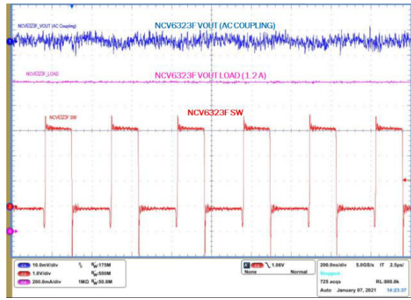
Figure 52. Output Voltage Ripple ( V_{IN} = 3.3 \text{ V} , V_{OUT} = 1.1 \text{ V} , C_{OUT} = \text{GCM21BR70J106KE22} , I_{OUT} = 500 \text{ mA} )
