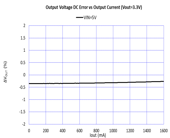
Figure 34. Output Voltage DC Error vs Output Current ( V_{OUT} = 3.3 V , T_A = 25^{\circ}C )
