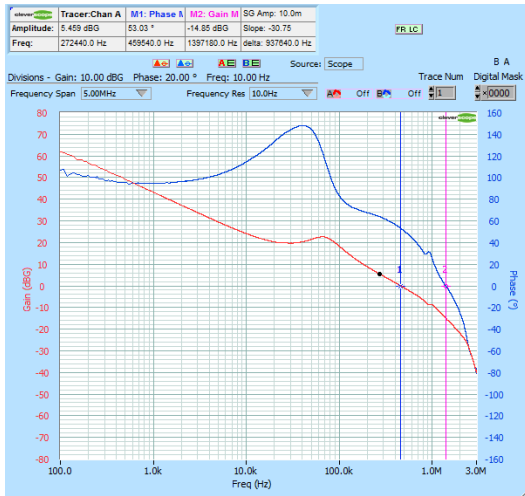
Figure 74. Bode Plot NCV6323FxmLMTW10TBG L = 1.0 \mu H – COUT = 10 \mu F
