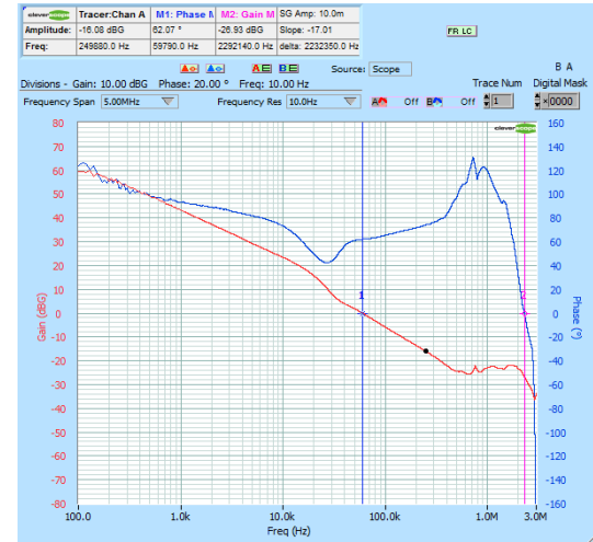
Figure 71. Bode Plot NCV6323FxmLMTW33TBG L = 1.0 \mu H – COUT = 100 \mu F
