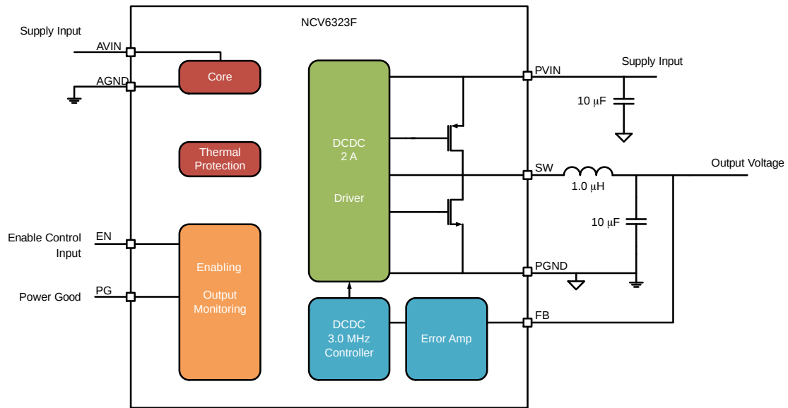
Figure 1. Application Schematic
