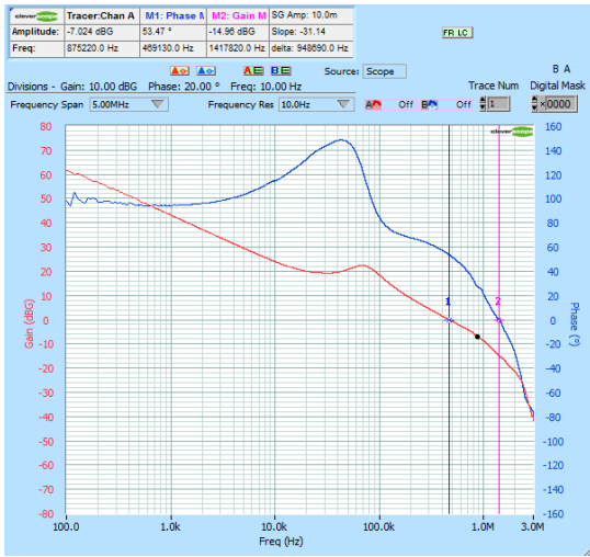
Figure 68. Bode Plot NCV6323FxmLMTW18TBG L = 1.0 \mu H – COUT = 10 \mu F
