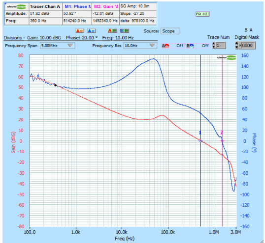
Figure 70. Bode Plot NCV6323FxmLMTW33TBG L = 1.0 \mu H – COUT = 10 \mu F
