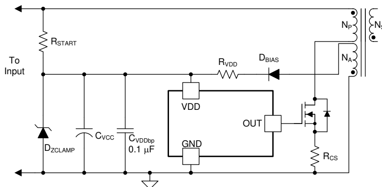
Figure 7-1. VDD Protection
