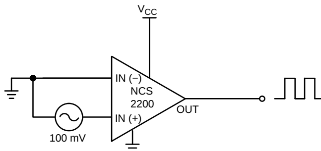
Figure 21. Zero-Crossing Detector
