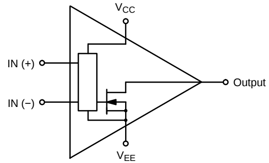
Figure 17. NCS2202/NCS2202A Open Drain Output Configuration
