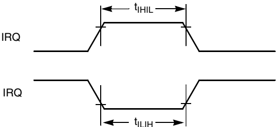
Figure 5. IRQ Timing
