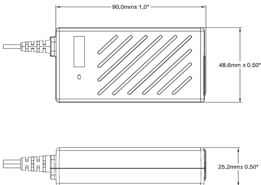
IPD30-Class I-DWG
